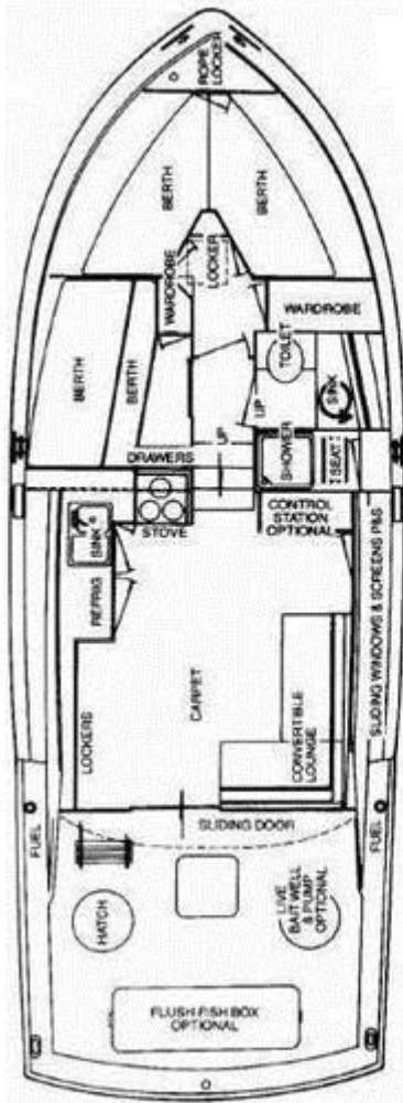
STOCK FLOORPLAN
