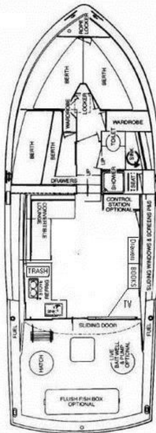
FLOORPLAN B
