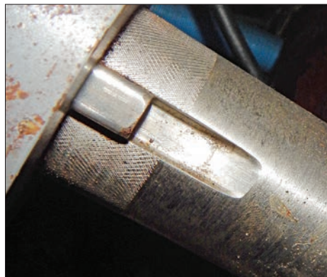
Left —A ramped and radiused keyway is more resistant to stress-induced fractures, while the knurling improves the interference fit on this small sail auxiliary straight-bore coupling. Right —Keys should fit snugly into a keyway and, when lightly oiled, should slide and be easily removed. Unlike this one, they should not rock or clack when moved from side to side.
